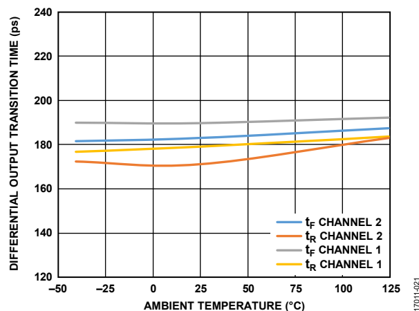
Figure 26. Differential Output Transition Time vs. Ambient Temperature
