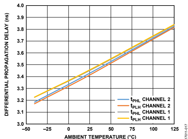
Figure 22. Differential Propagation Delay vs. Ambient Temperature
