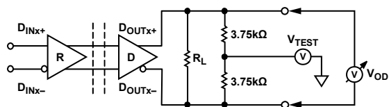
Figure 37. Driver Test Circuit (Full Load Across Common-Mode Range)
