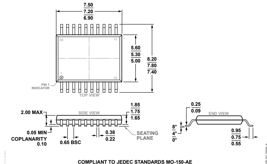
Figure 46. 20-Lead Shrink Small Outline Package [SSOP] (RS-20)
